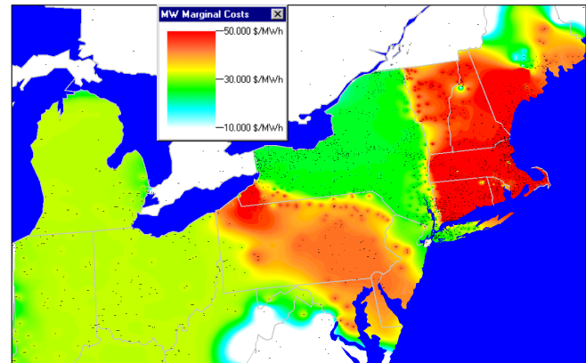
Figure 4: Contour of “Regulated” Bus Marginal Prices
