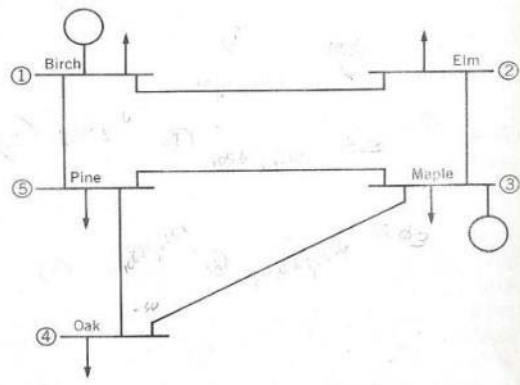
Figure 8.1 One-line diagram for Example 8.1.
