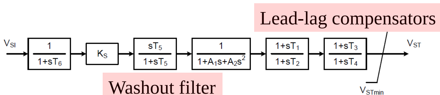
Figure 31 —Type PSS1A single-input power system stabilizer
